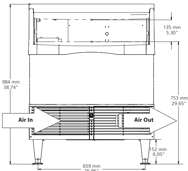
CU3030 front view
