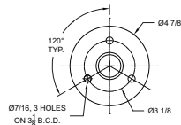
FOOT DETAIL "A"
