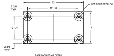
BASE MOUNTING DETAIL
