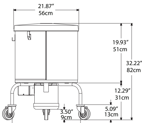
Side View SALD-1, SALD-2
