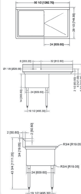
ONE TUB SINK WITH RIGHT DRAIN BOARD
