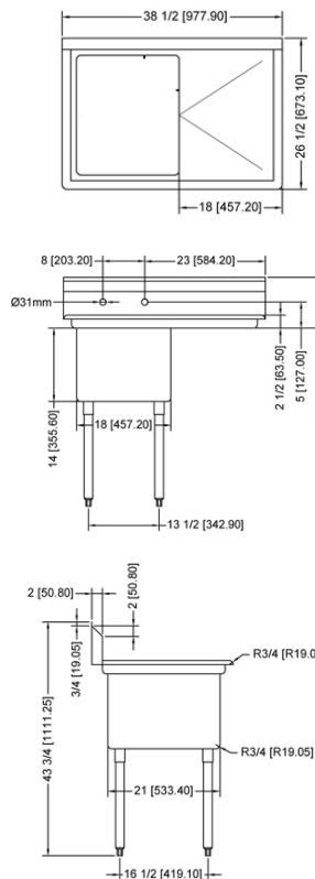
ONE TUB SINK WITH RIGHT DRAIN BOARD
