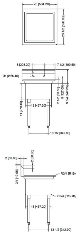
ONE TUB SINK WITHOUT DRAIN BOARD
