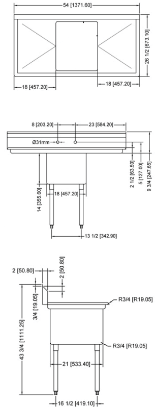
ONE TUB SINK WITH TWO DRAIN BOARD
