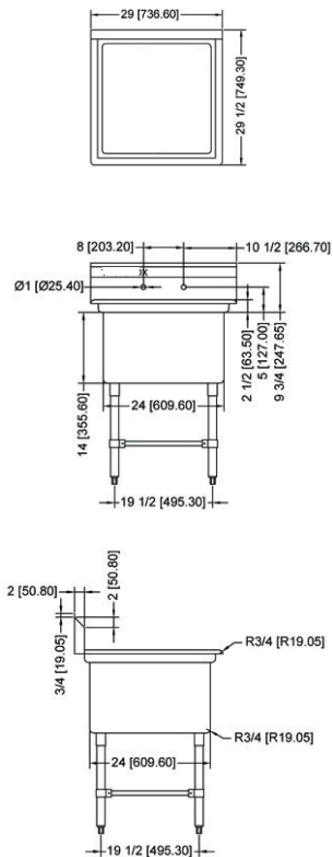
ONE TUB SINK WITHOUT DRAIN BOARD
